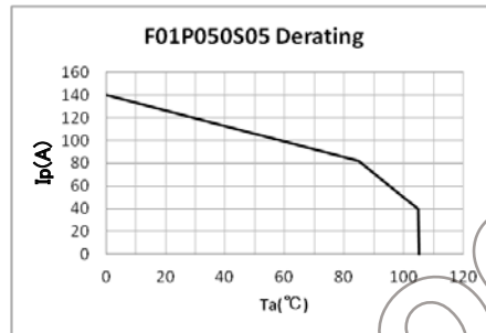
Figure 6: Ip vs Ta for F01P050S05
