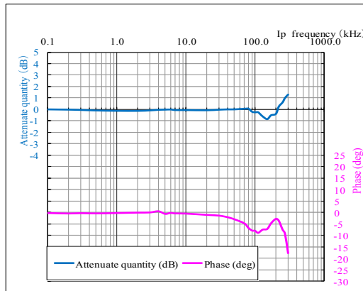
Figure 2: Frequency response curve
