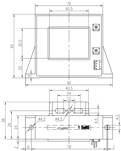
NACF.800J1-S5/V 电压传感器外形图 Dimensions NACF.800J1-S5/V Series (in mm)
