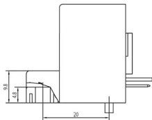
NACF.50C-S5/V 电压传感器外形图 Dimensions NACF.50C-S5/V Series (in mm)
