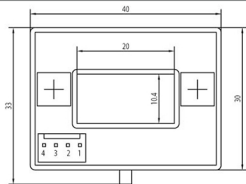
NACF.50C-S5/V 电压传感器外形图 Dimensions NACF.50C-S5/V Series (in mm)
